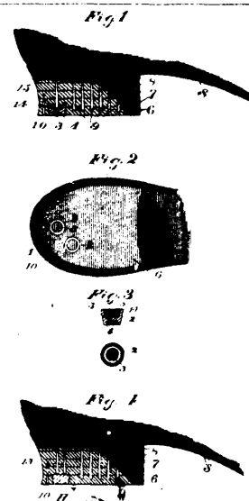
27073 Hull's Heel Protector.
