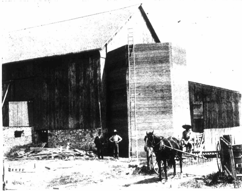
CEMENT SILO OF MR. JAMES BEGG, ST. THOMAS. Size: 11 feet inside diameter; 25 feet in height. Hexagon shape (6 sides). Built with BATTLE'S THOROLD CEMENT.
