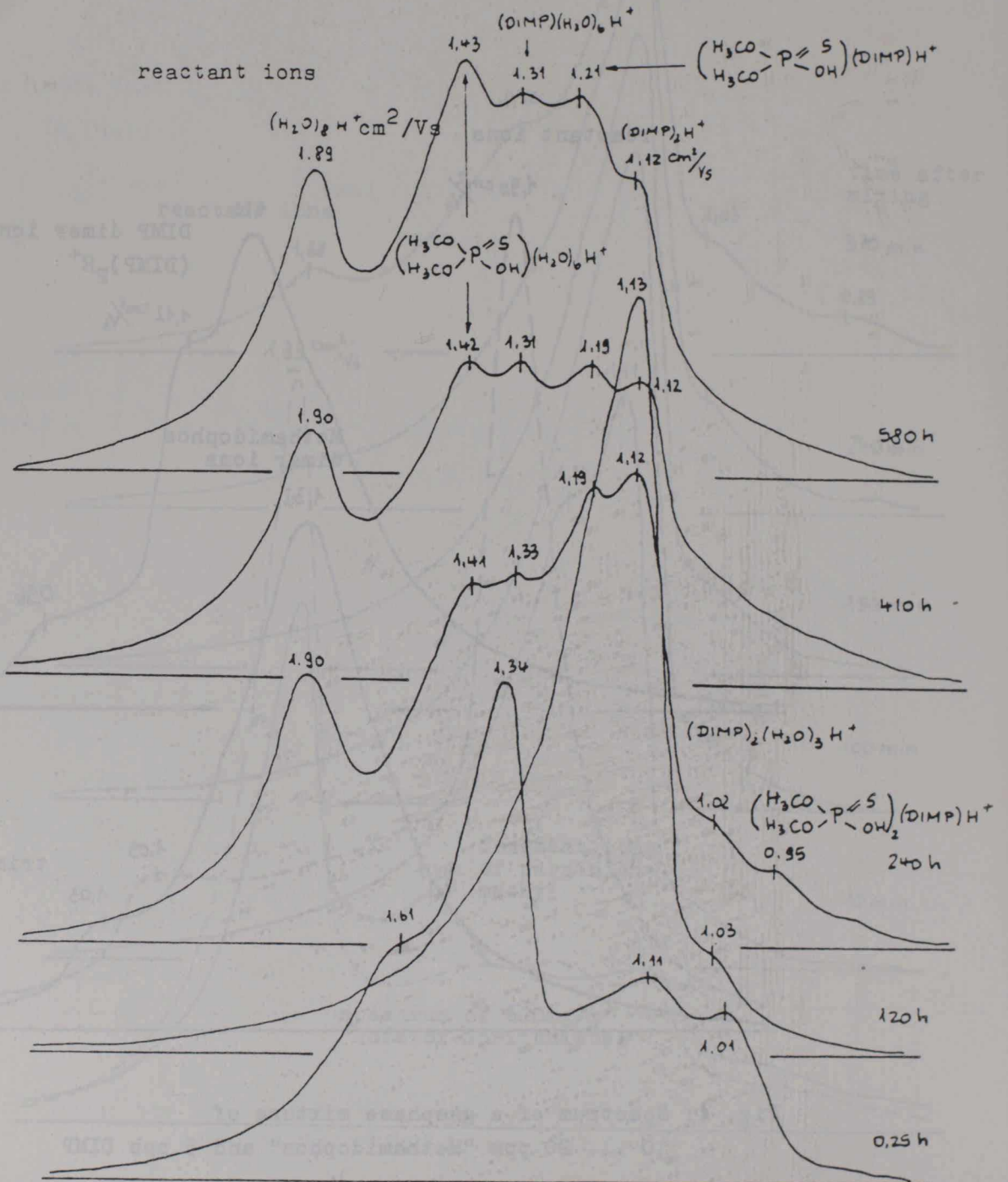
Fig. 5: Spectra recorded from a rubber sample contaminated with Wofatox + 1 o / 00 DIMP mixture, with increasing storage time
