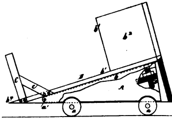
4819 Foster's Railroad Snow-plough.
