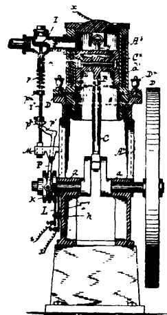
39260 Barrett and Daly's Gas Engine.
