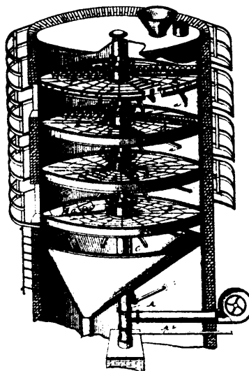
33221 Gent's Drying Apparatus.
