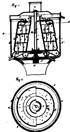
33217 Wahl's Butter Extractor.
