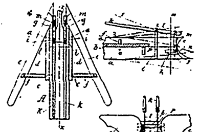
30070 Sloat's Machine for Sharpening Harrow Disks.
