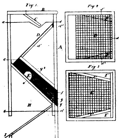
18701 Cameron's Cider Sifter.
