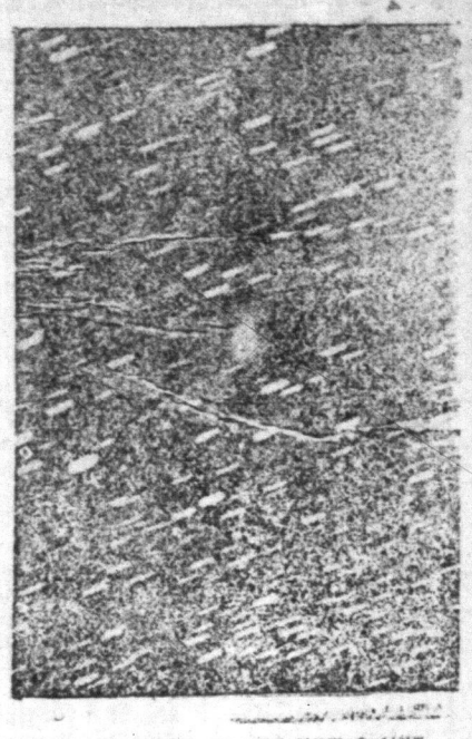
PHOTOGRAPH OF THE NEW COMET. The comet is the white blur in the centre of the picture. The long dashes of white were made by the motion of the stars.
