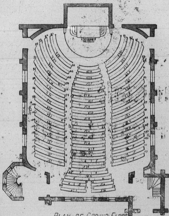
PLAN OF GROUND FLOOR
