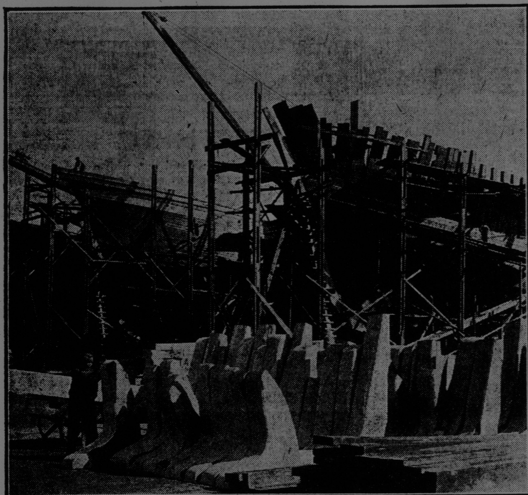
A GROUP OF PERFECT KNEES, NATURAL GROWTH—Trunk and main root of trees adapted to support decks in building of wooden ships in Vancouver Island.
