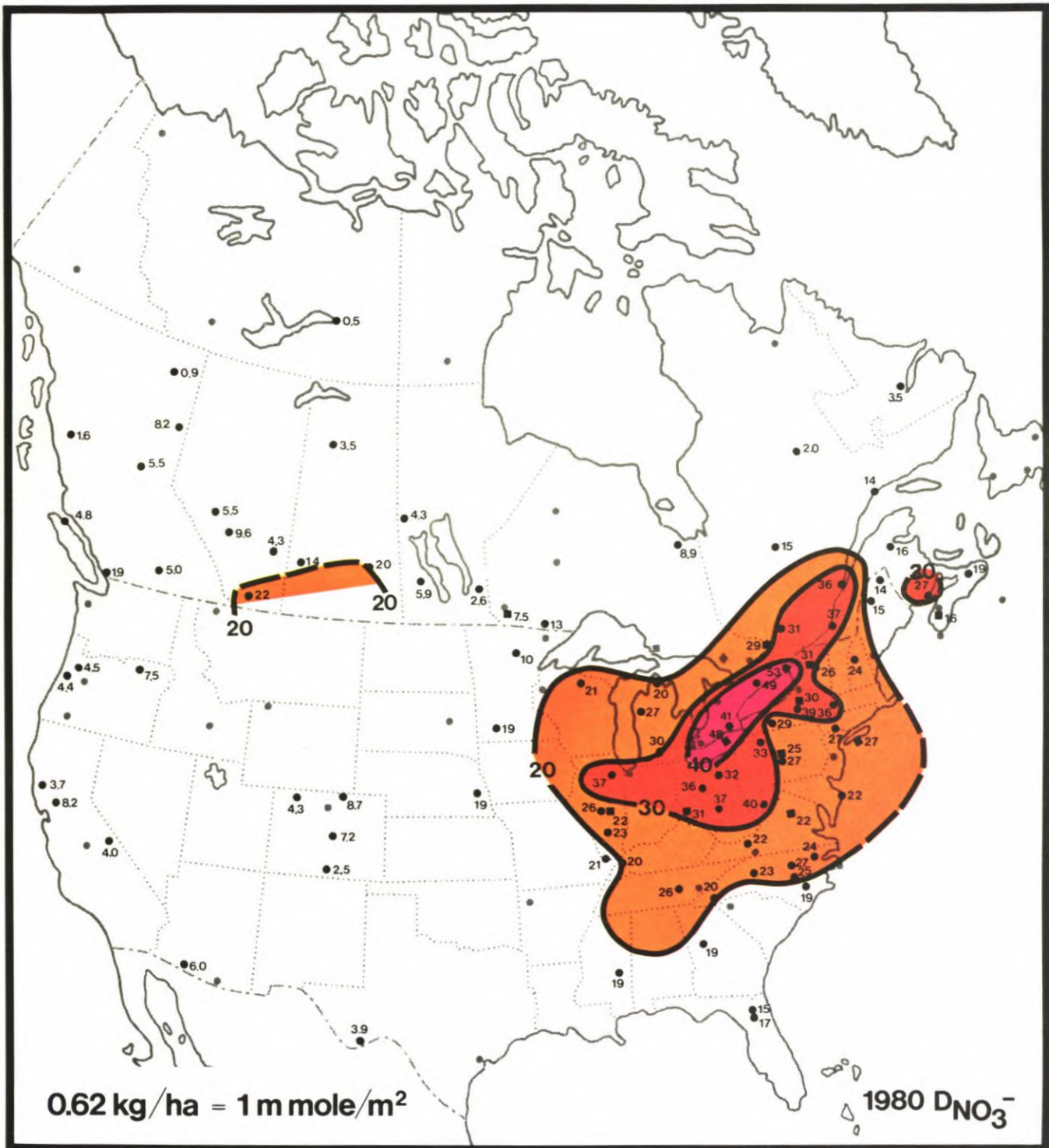
Precipitation amount- weighted mean nitrate ion deposition for 1980 (m moles per square meter)
