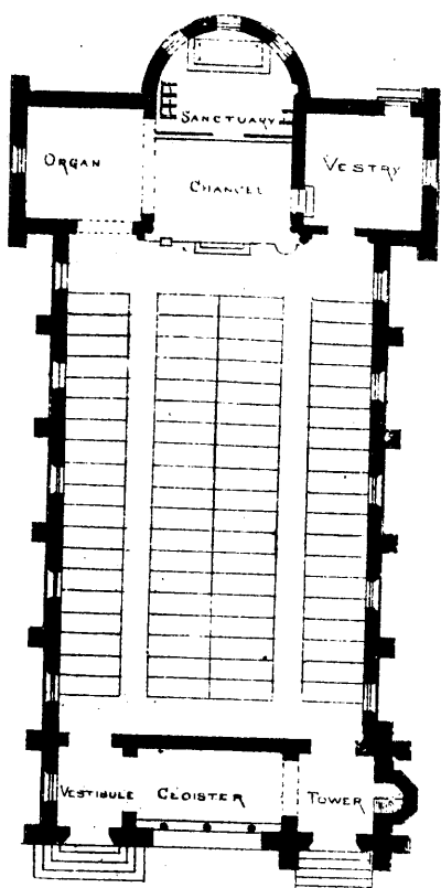
GROUND PLAN
