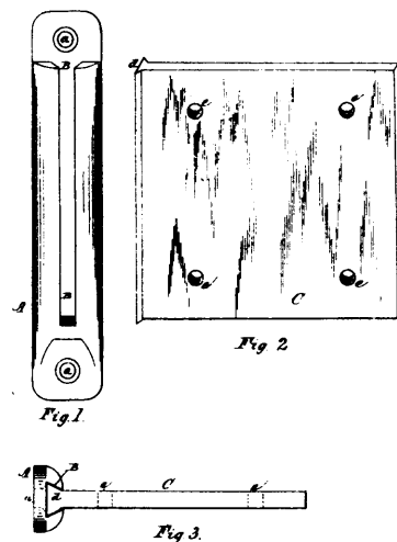
38960 Darby's Bedstead Lock.
