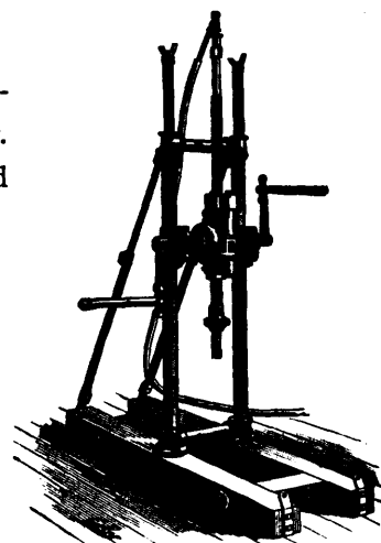
"BRAVO" Hand Power Drill HOLE, 350 FT. DEEP. CORE, 1 3/4-16 IN. DIAMETER.
