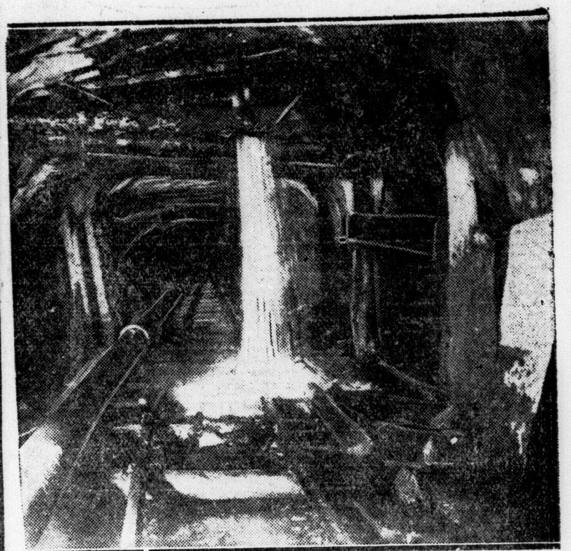
A leak in the Simplon tunnel, running under the Alps from Switzerland to Italy, which is approaching completion. Work was begun nearly 20 years ago. Hydraulic pressure is used for drilling purposes and breaks in the water mains sometimes occur.
