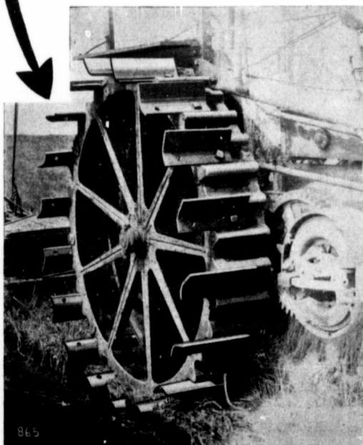
Cut shows how "Hold Fast" lugs grip the ground and pull out straight away without tearing up soil.
