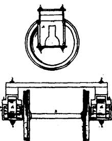
10180 Blakeley's Improvements on Car Axle Boxes.
