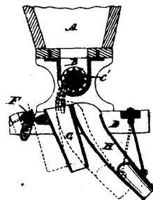
10164 Noxon's Improvements on Seeders.
