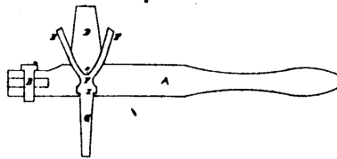
8602 Harris' Die and Swage for Making King Bolts.
