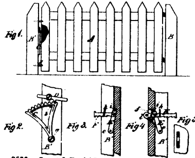
8596 Sweet &amp; Davis' Improvements on Doors and Gates.
