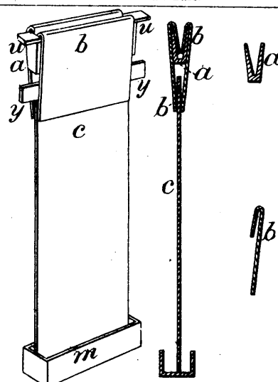
16066 Nichol's Improvements in Apparatus for Evaporating or Concentrating Liquids, and Saturating Liquids with Gases.
