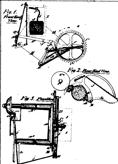
16069 Appleby's Improvements in Grain Binders.
