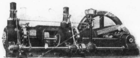
WARREN TANDEM ENGINE. Sizes to 1,000 H.P. Engines of this type operating within a short distance of Toronto have established World's Records for Reliability and Fuel Economy .
