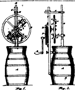
5157 Guest's Churn Power.
