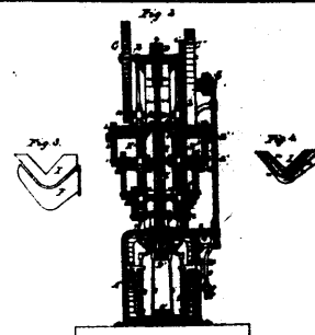
5162 Long's Leather Crimping Machine.
