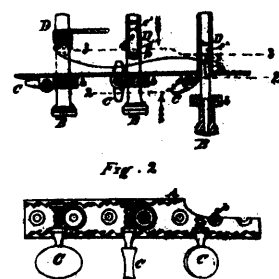
5165 White's Guitar Head.
