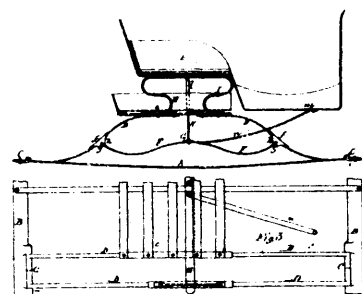
3145 Murgatroyd's Improvements in Carriage Springs.
