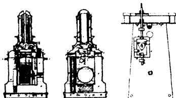
3138 Hitchcock's Forced Blast Heavy Oil Lamp.
