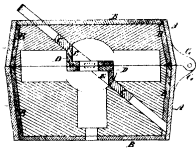
3137 Parker's Improvements on Moulds for Casting Cores.
