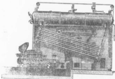
"B. & W." PATENT WATER TUBE BOILER. SUPERHEATER AND IMPROVED STEAM AND STOKER.
