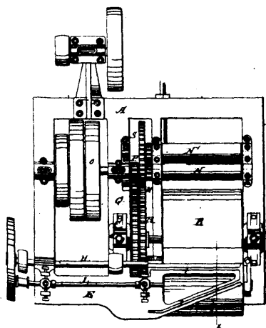
19197 Davis's Machine for Cleaning Intestines.
