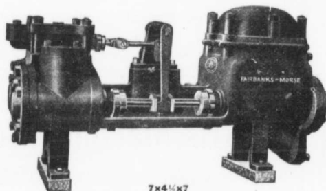
DUPLEX PISTON PATTERN PUMP
