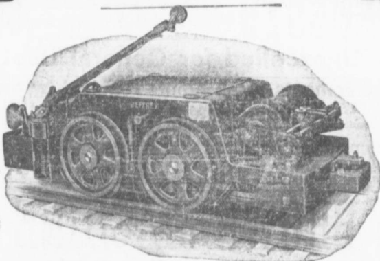
JEFFREY S. M. 15, 2½ ton Electric Gathering Locomotive with —outside Wheels.—
