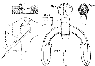
11641 Martin's Improvements on Anchors.
