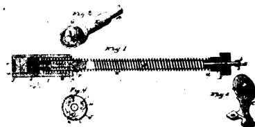
11628 Noyes's Improvements in Curtain Rollers.
