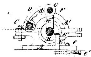
11622 Anderson's Improvements in Machines for Cutting Springs.
