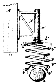
11636 Schoen &amp; Scott's Improvements on Furniture Castors.
