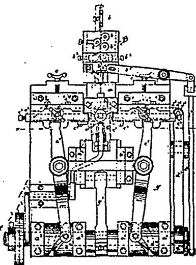
24365 Hassall's Machine for Making Wire Nails.
