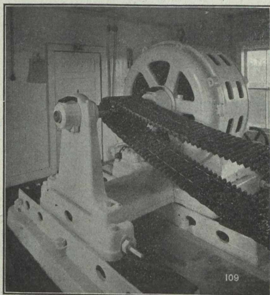
Two views (full view unobtainable owing to cramped space) of a 150 h.p. Renold Chain Drive from Motor to Sturtevant Blower. Shaft centres 8½ ft. (Minimum permissible by proportions of apparatus). Driven sprocket is of special side spring cushion type construction to absorb the impulses of the load.
