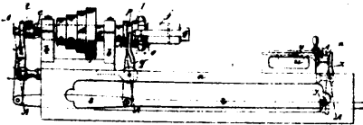
No. 1713. Laurie's Bolt Cutting Machine.
