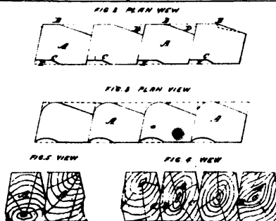
No. 1722. Ballard's Wooden Pavement.
