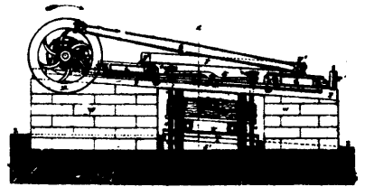
No. 1710. Young's Stone-Cutting Machine.
