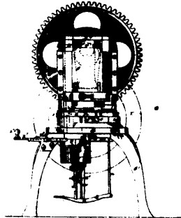
No. 1714. Bigelow's Boot and Shoe heel compressing machine.
