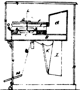
No. 1717. Thornton's Improved Cabinet Organ.
