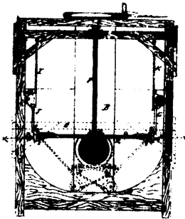
No. 1715. Marshall's Wood bending machine.
