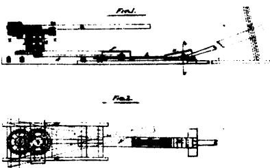
No. 1721. Strong's Improved Horse Power.
