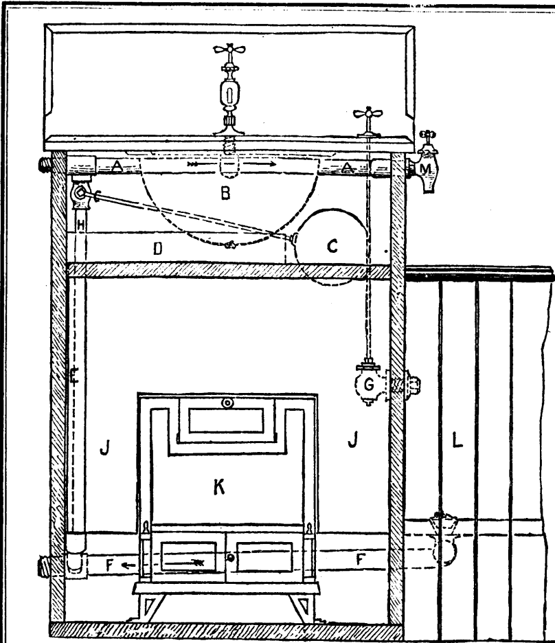
PORTABLE BATH TUB AND WASHSTAND.—FIG. 2.—SECTION SHOWING THE WORKING PARTS.
