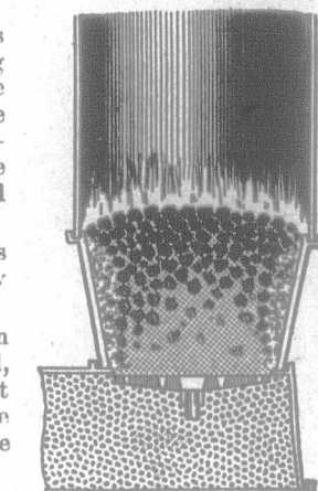
Ordinary Fire-pot.
