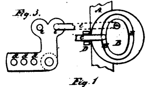
11876 McKenzie's Improvements on Fanning Mills.
