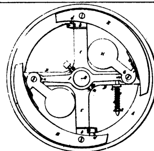
5119 Heebner &amp; Seipt's Governor for Horse-power.
