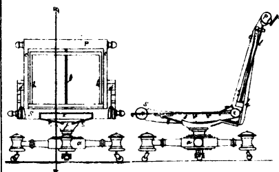
5115 Roy's Invalid Chair.
