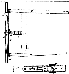
5117 McIntosh &amp; Boyce's Shaft Support.
