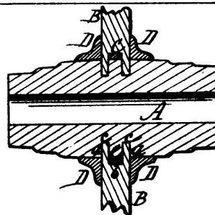
5109 Mitchell's Carriage-hub.
