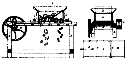
5110 Burn's Root-cutter.
