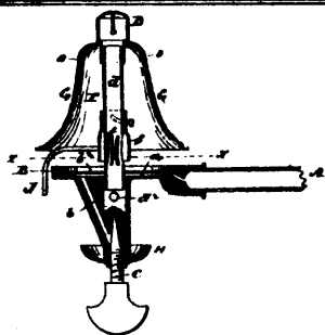
5104 Benson's Vapour-burner.
