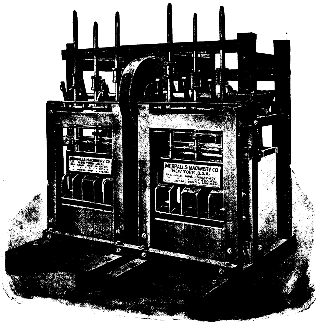
A SIX STAMP BATTERY
