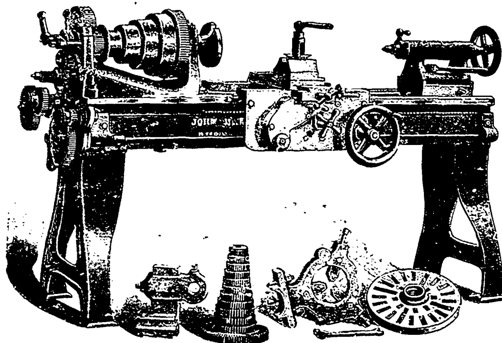
16-in. LATHE;
