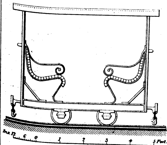
Fig. 20. Inspector's Carriage for Channel Tunnel.
