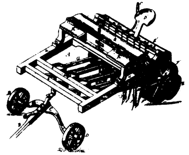
6452 Holland's Combined Land Roller and Seeding Machine, &amp;c.
