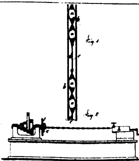
6460 Bailey's Tubular Flues for Steam Boilers.
