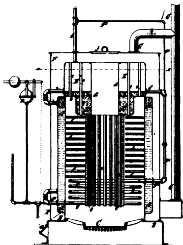
27462 Steele's Steam Boiler.
