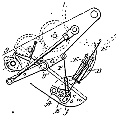
25429 Bullock's Grain Binder Attachment.
