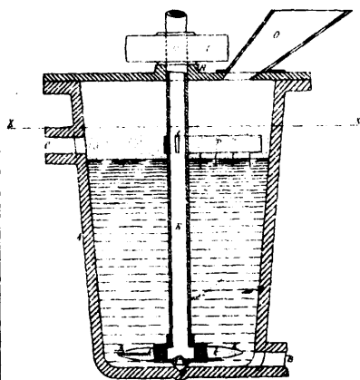
17487 Huntington and Koch's Amalgamating Apparatus.
