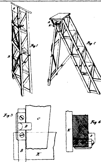
17493 Jones' Steps or Self-Supporting Ladder.
