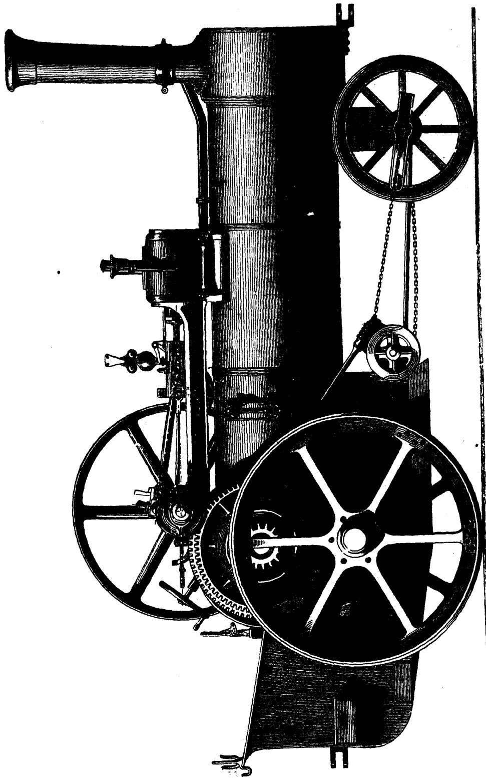
SIX-HORSE POWER TRACTION ENGINE.—END VIEW. (See page 69.)
