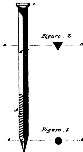
16407 Taylor's Improvement in Nails or Spikes.
