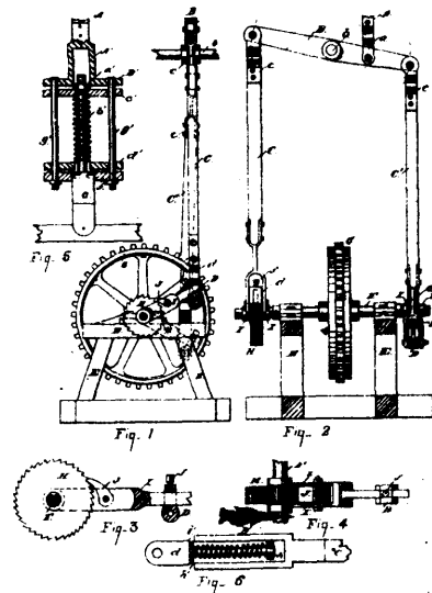
16404 Croft's Improvements on Power Converters.
