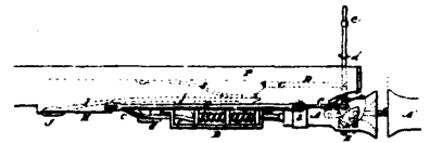
2948 Knowlton's Car-coupling.
