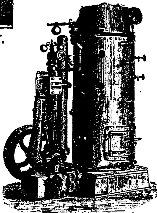
VERTICAL AND MARINE ENGINES AND BOILERS.
