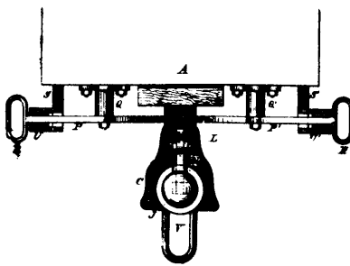
8425 Dette, Cohen and Millring's Improvements on Car-Couplings.
