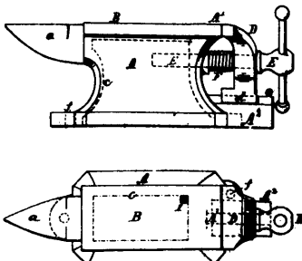
8442 Parker and Curtis' Improvements on Combined Anvils and Vises.
