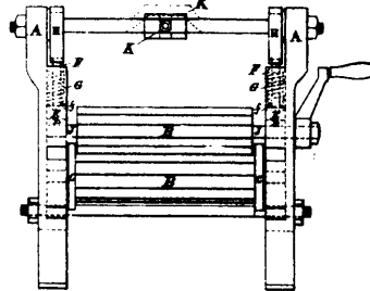
8433 Fee and Cable's Improvements on Clothes Wringers and Washing Machines.
