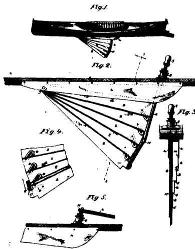
Childs' Folding Centre Board.
