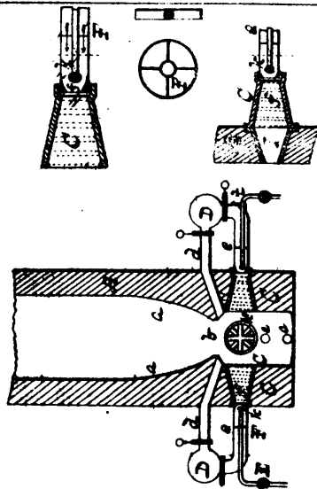
18921 Morgan & Hayden's Reducing and Smelting Metals and Furnace Therefor.
