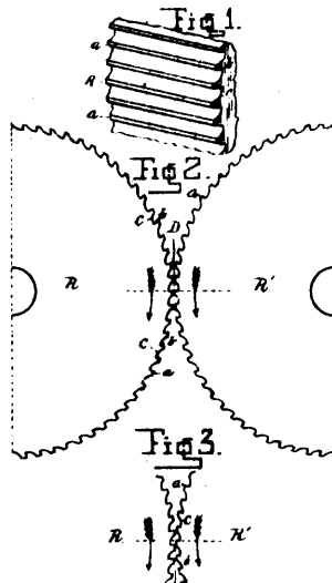
18922 Rickerson's Roller Mill.
