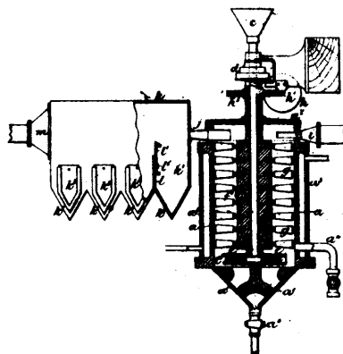
18925 Jordan's Apparatus for Treating Ores Chiefly for the Extraction of Precious Metals Therefrom.
