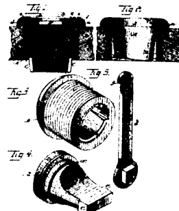
15353 Jackson's Improvements on Bushes and Bungs.
