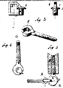
15349 Hunter's Improvements on Harness and Trace Couplings, Neck Yokes and Pole Clips.
